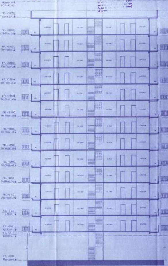
SECTION Y-Y
