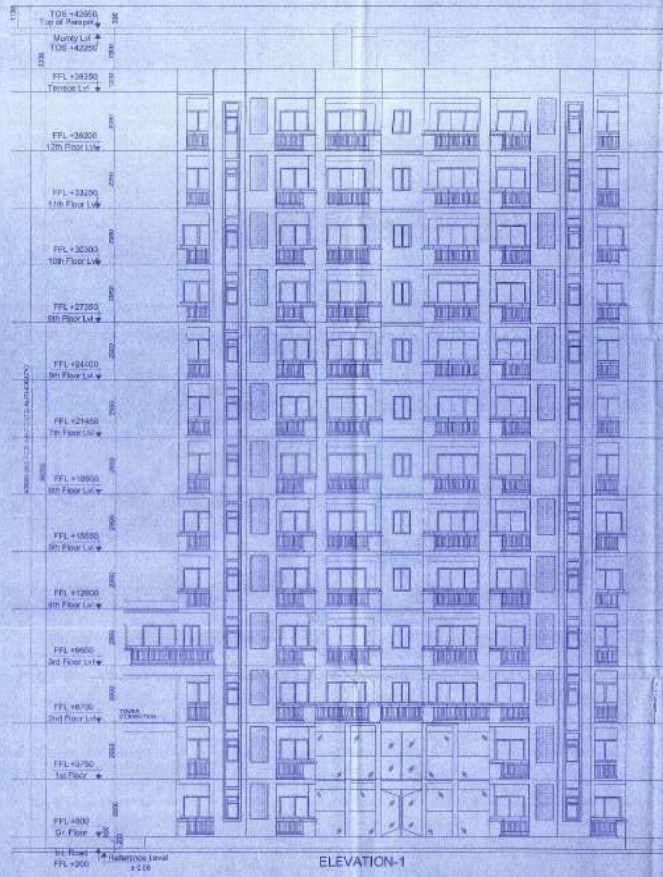
ELEVATION-1
