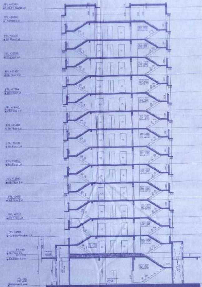
SECTION X-X
